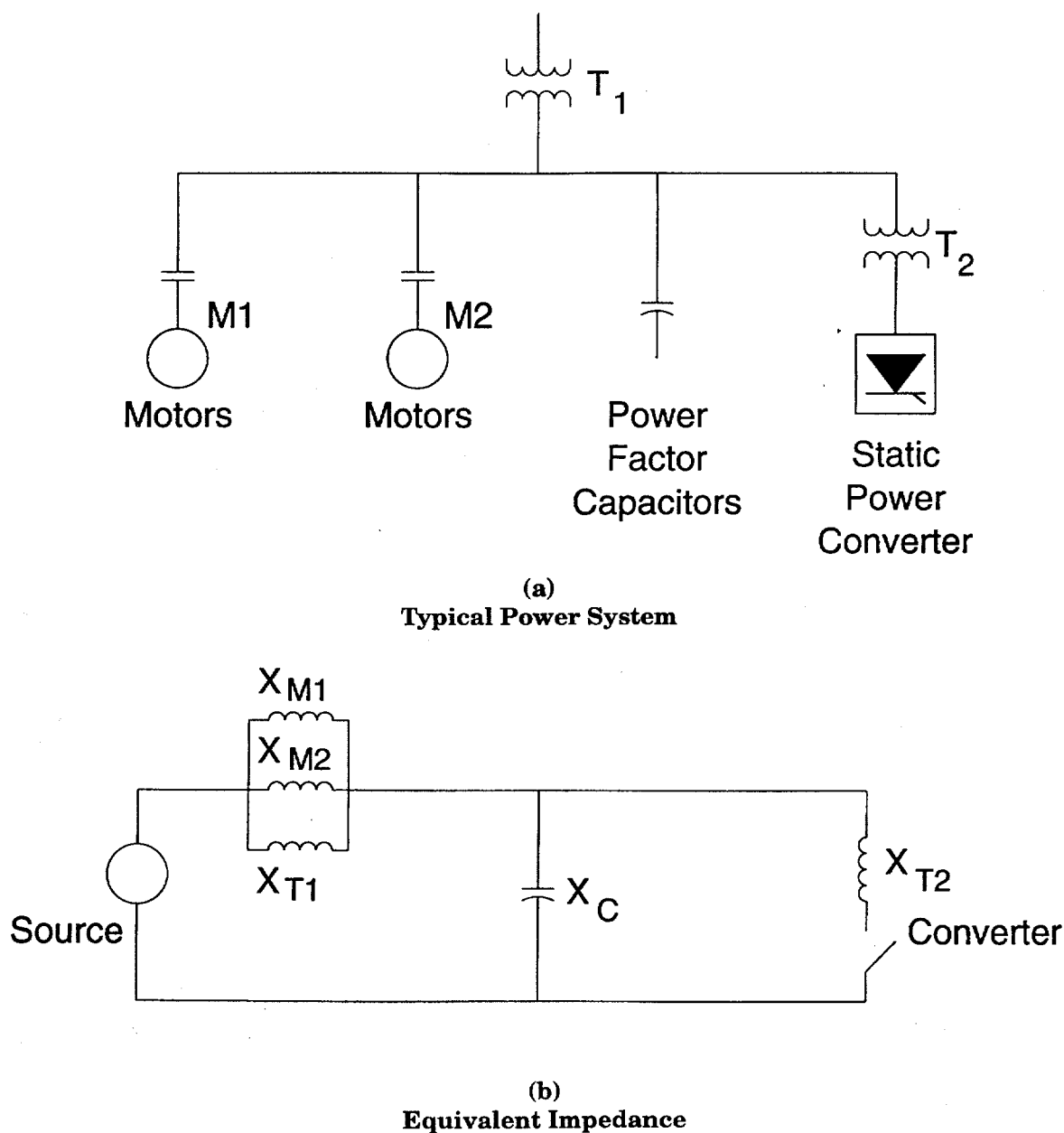
Figure 8-7—Typical Power System and Equivalent Impedance Diagrams
